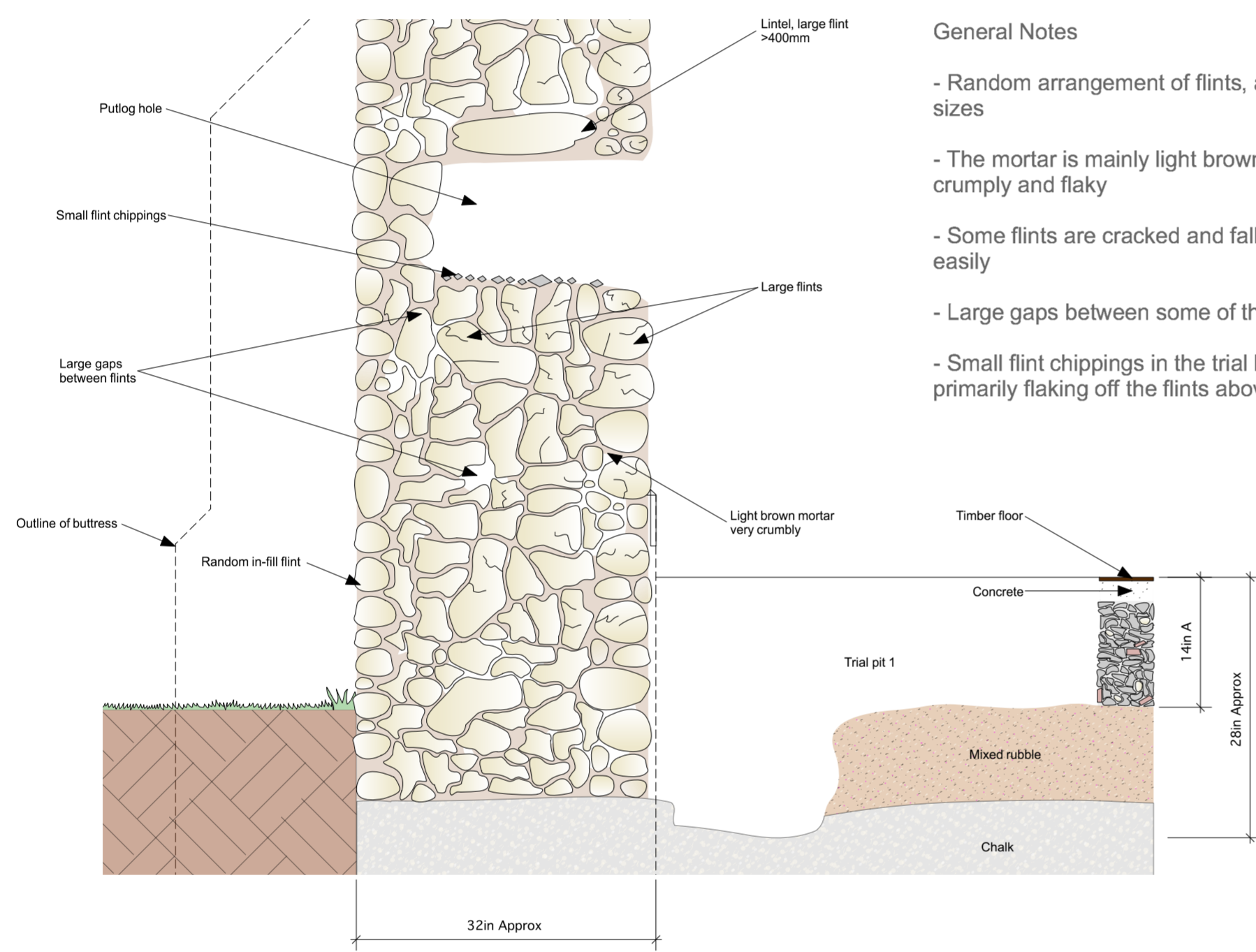
Section BB
