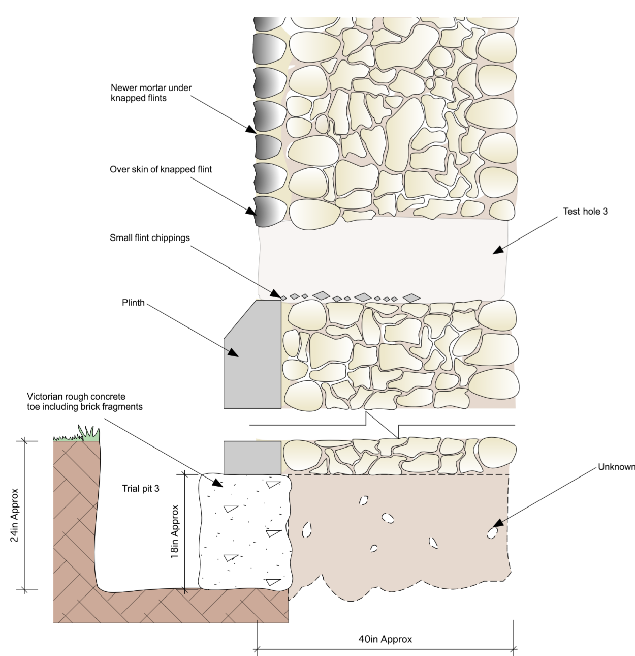
Section CC
